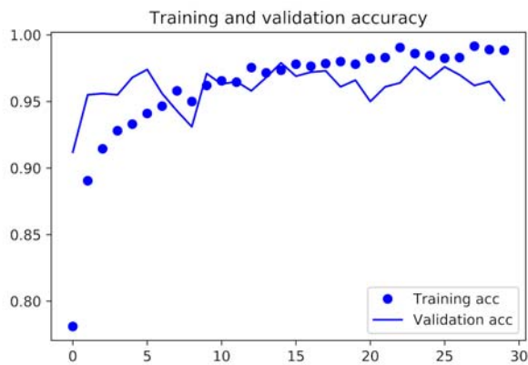
Figure 5.20 Training and validation accuracy for fine-tuning
