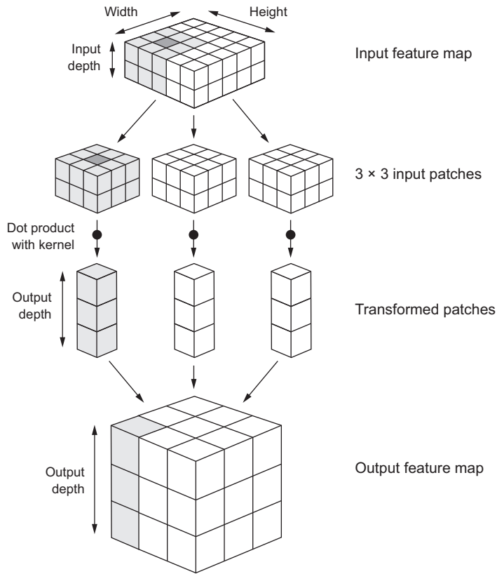
Figure 5.4 How convolution works
