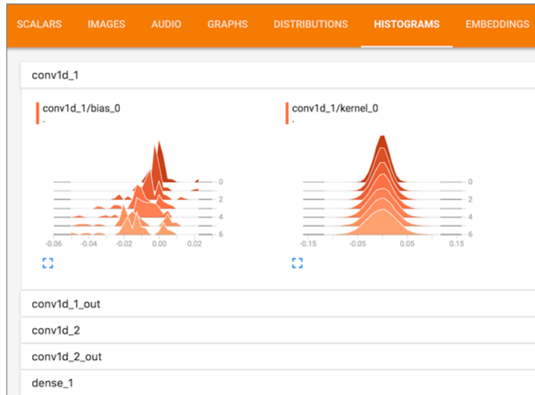
Figure 7.11 TensorBoard: activation histograms
