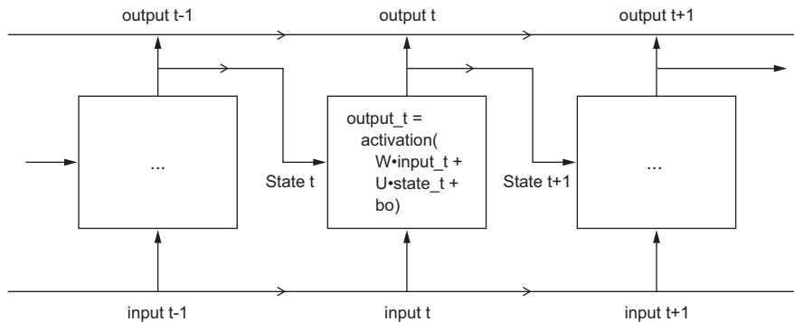
Figure 6.10 A simple RNN, unrolled over time
