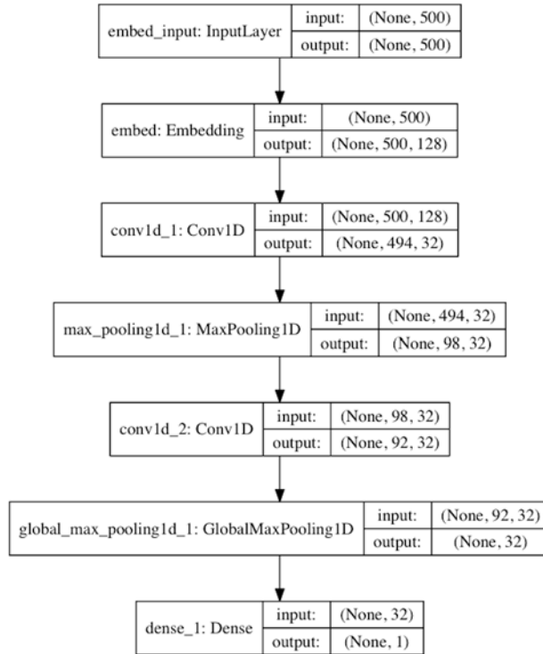
Figure 7.15 A model plot with shape information
