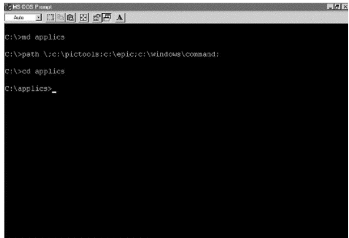
Figure 2.7 Creating applies directory and using the path DOS command.
