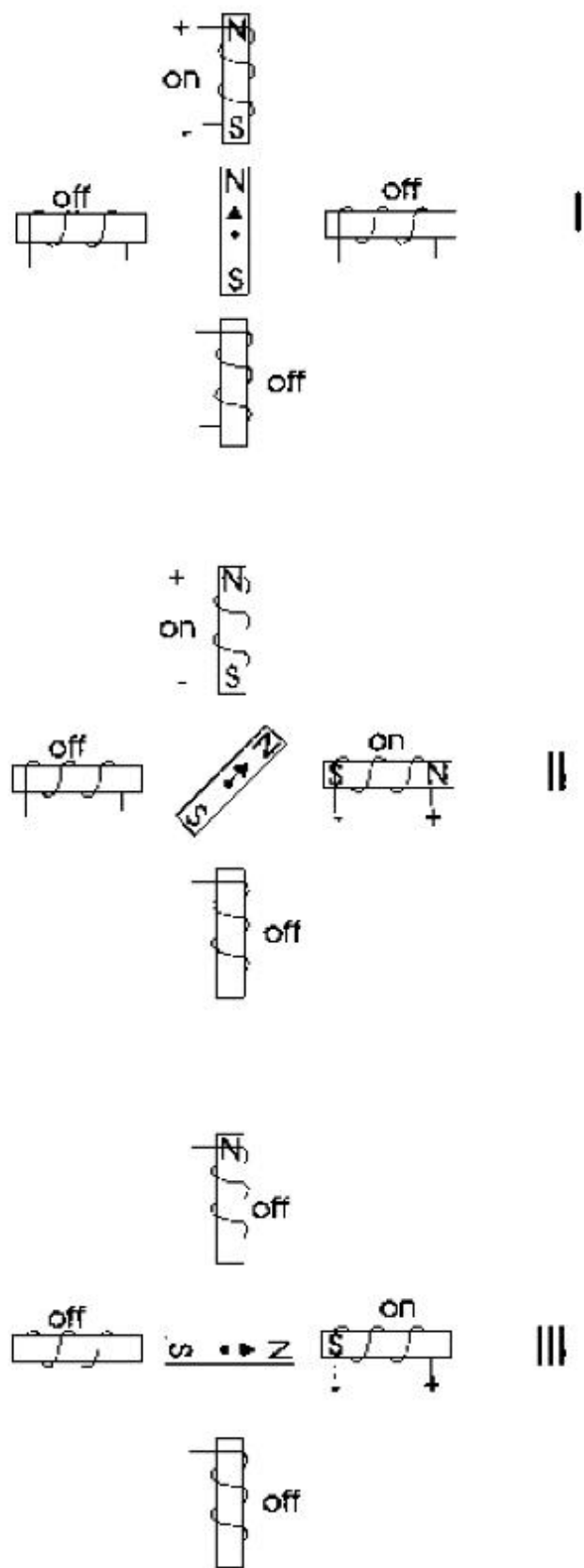
Figure 12.2 Half-stepping.
