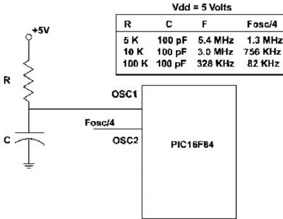
Figure 6.3 RC oscillator.
