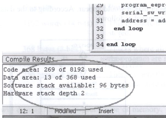
Figure 119. Compiler result.
