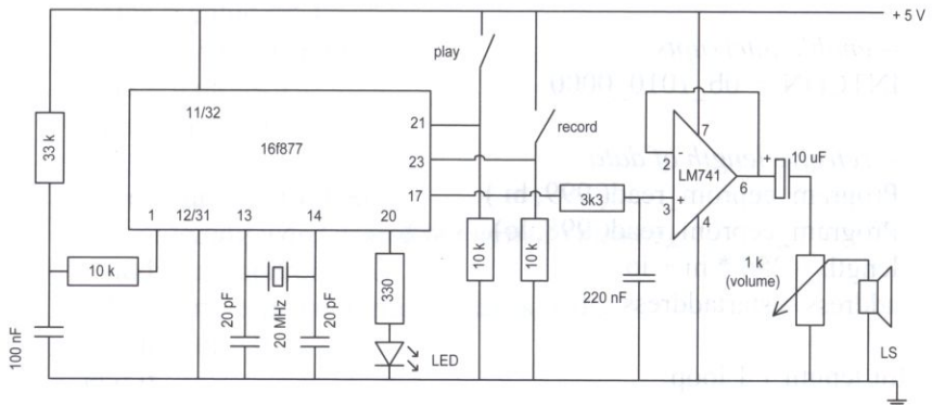
Figure 114. Super compression.
