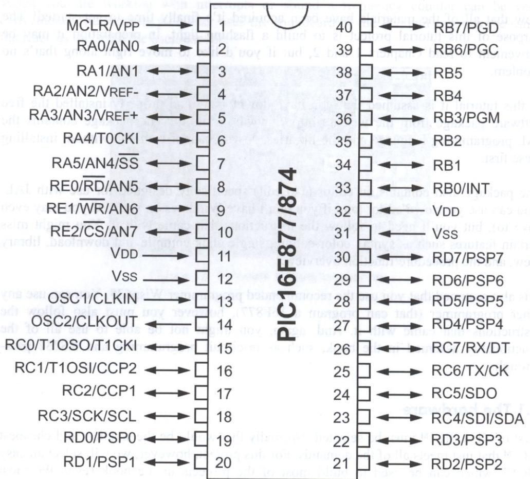
Figure 16. Pin layout for 16F877.
