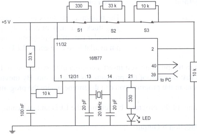
Figure 51. Silent alarm with a single wire loop.
