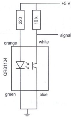
Figure 70. Connecting the QRB1134.
