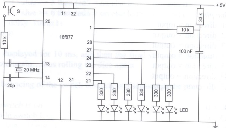
Figure 29. Electronic dice.
