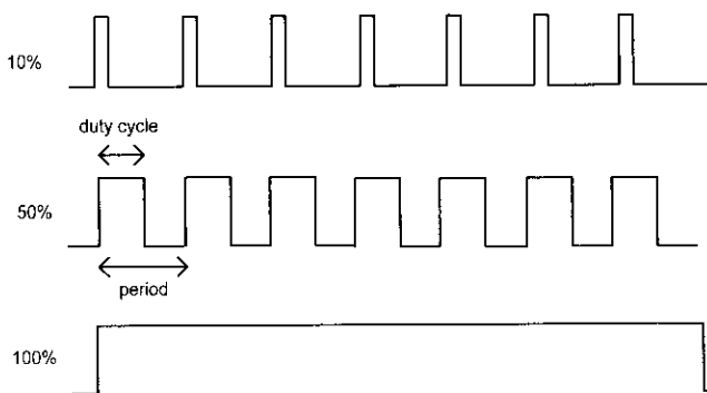
Figure 62. PWM duty cycles.
