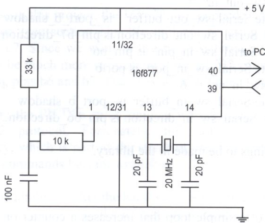
Figure 46. Serial counter.
