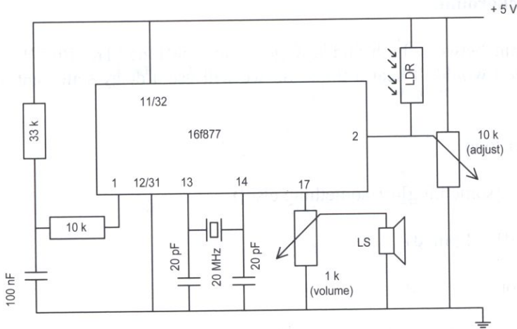
Figure 101. Night buzzer.
