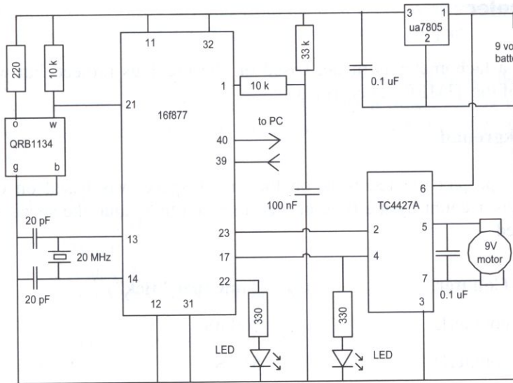
Figure 74. Constant speed with feedback.
