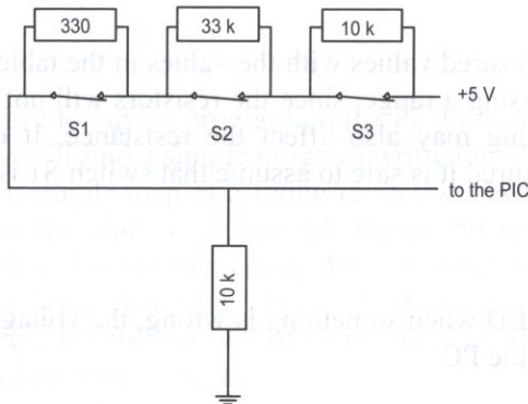
Figure 49. Voltage divider.
