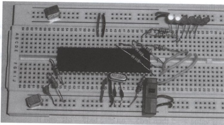
Figure 30. Electronic dice.
