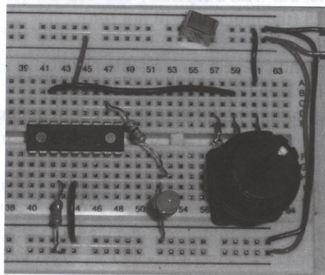
Figure 202. Adjustable clock frequency.
