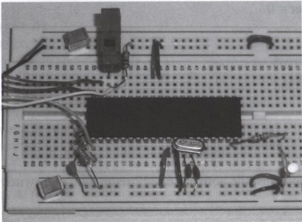
Figure 152. Port B interrupt on the breadboard.
