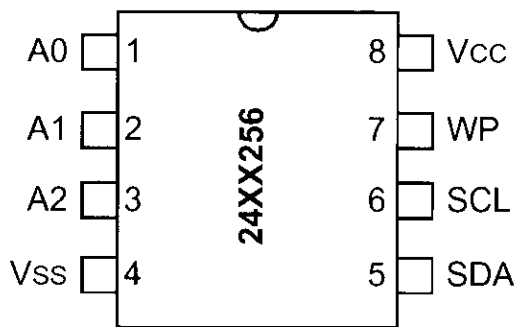
Figure 128. Pin configuration.
