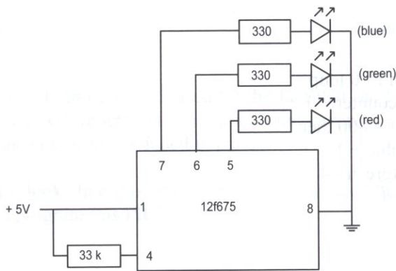
Figure 191. RGB fader.
