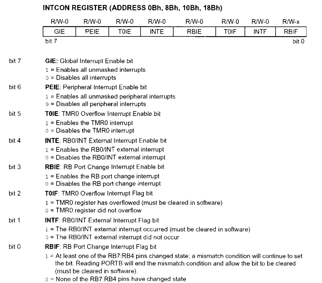
Figure 150. INTCON register.
