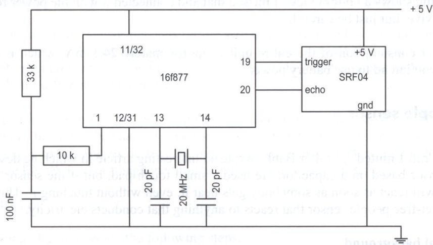
Figure 86. Ultrasonic sensor.
