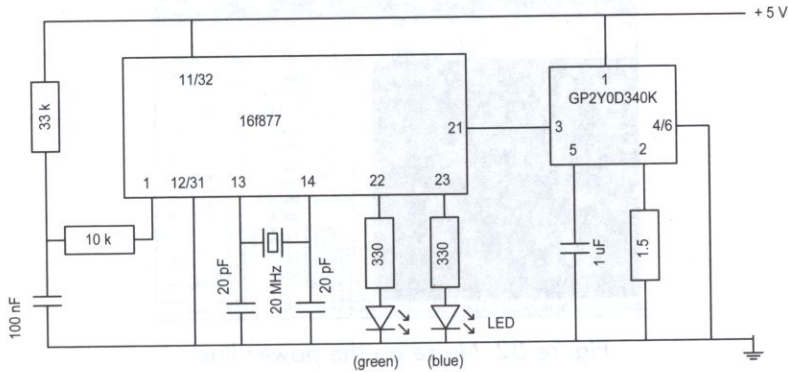
Figure 80. Infrared sensor.
