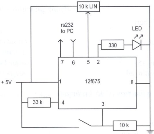
Figure 186. Demo program for the 12F675.
