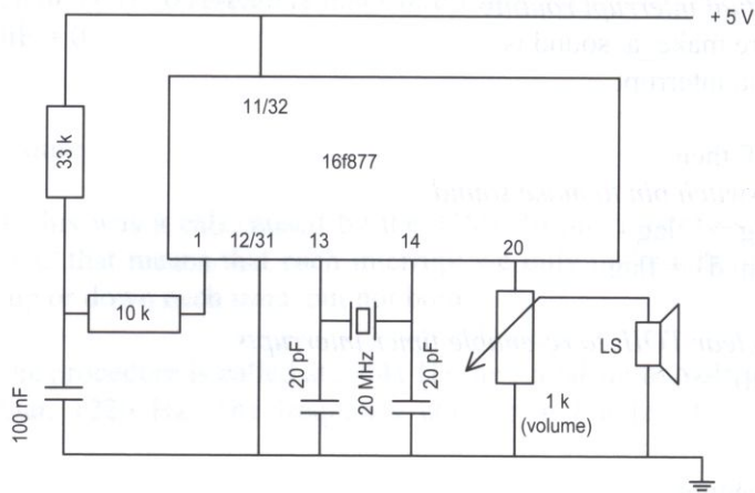
Figure 143. TIMER0 whistle.
