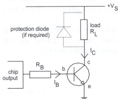
Figure 172. NPN transistor.
