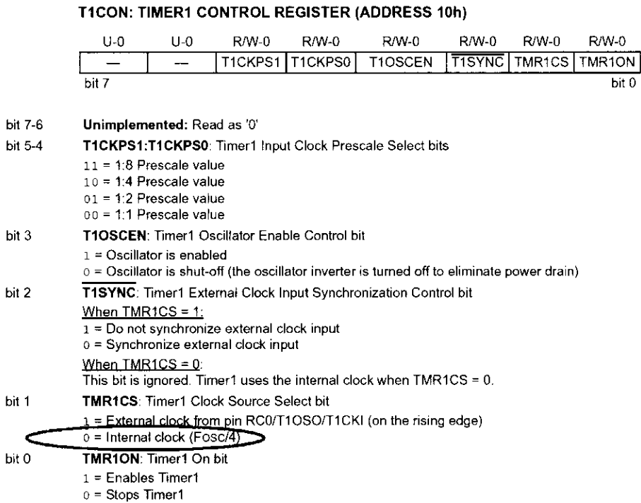
Figure 72. TIMER1 control register
