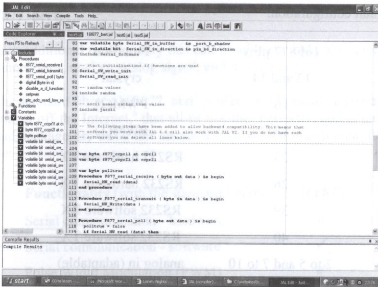
Figure 6. JALedit.
