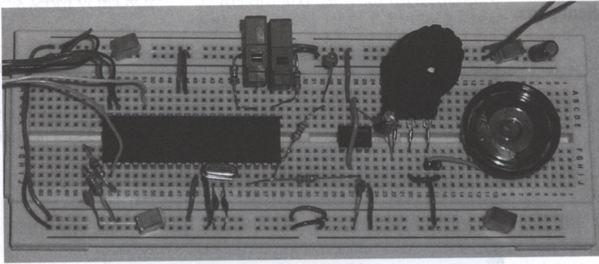
Figure 115. Super compression.
