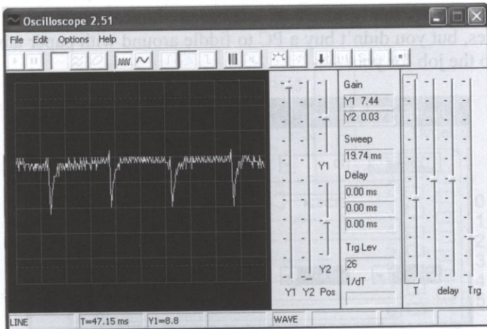
Figure 9. Software Oscilloscope.
