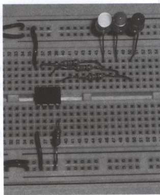
Figure 192. RGB fader.
