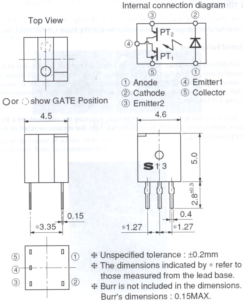
Figure 93. Datasheet for the tilt sensor, bottom view.
