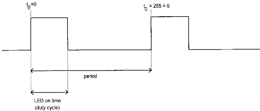
Figure 190. DIY PWM.
