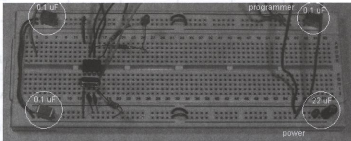
Figure 2. Breadboard with decoupling capacitors.
