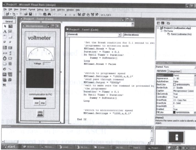
Figure 8. Visual Basic.
