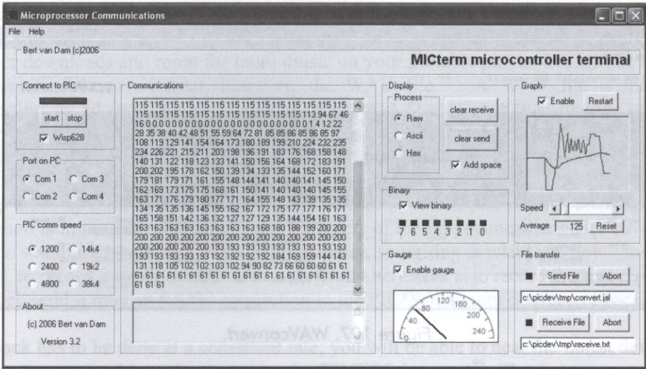
Figure 108. MICterm.
