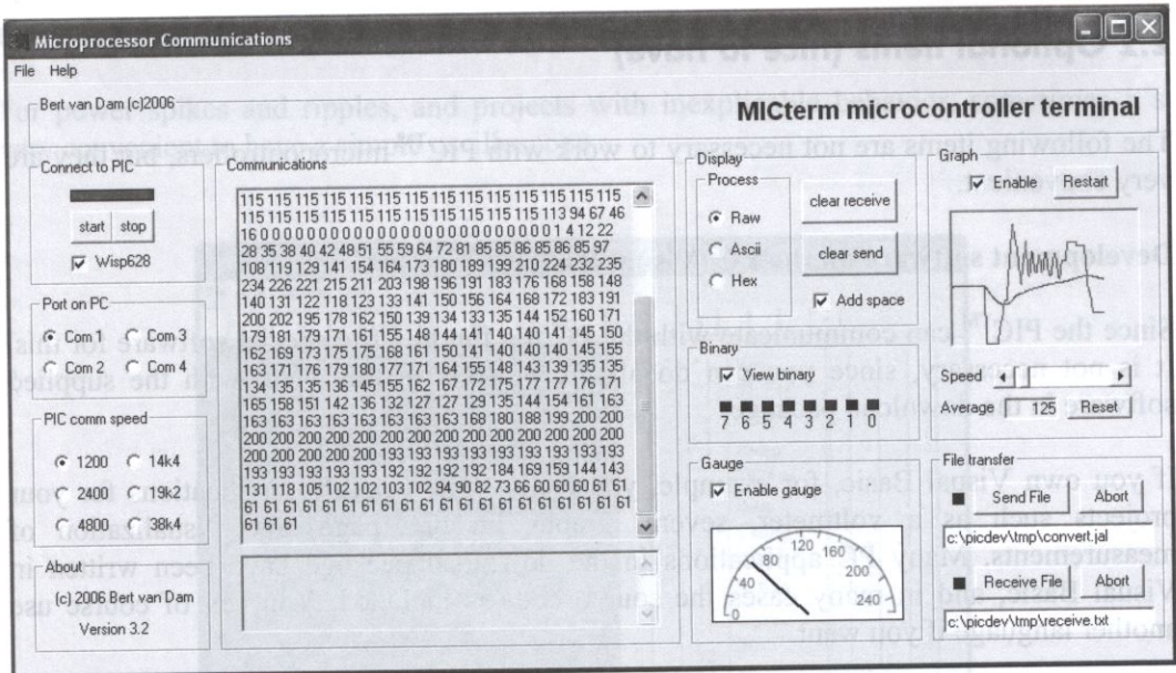
Figure 7. MICterm.
