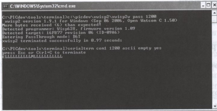
Figure 218. Serialterm started with a batch file.
