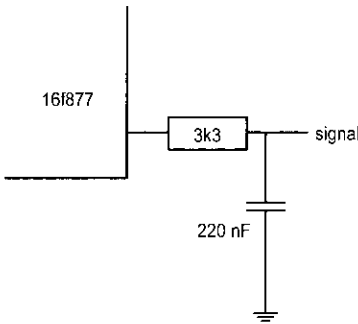
Figure 111. The RC network.
