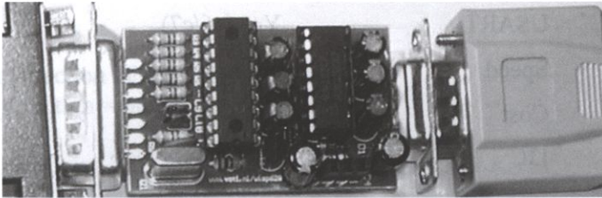
Figure 4. The Wisp628 in-circuit programmer.
