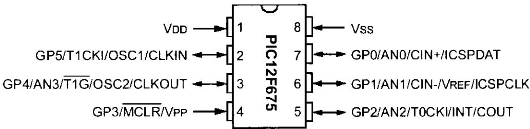
Figure 183. Pin layout of the 12F675.
