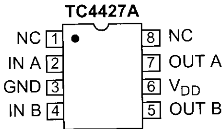
Figure 59. Pin layout of the TC4427A.
