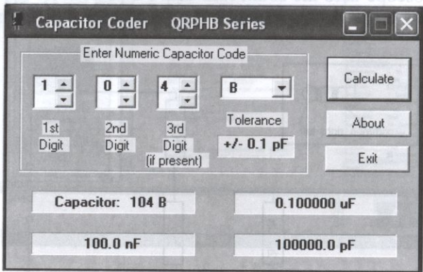
Figure 12. Capacitor coding.
