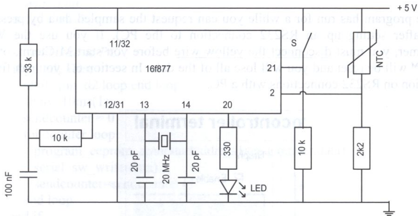
Figure 44. Sampling.
