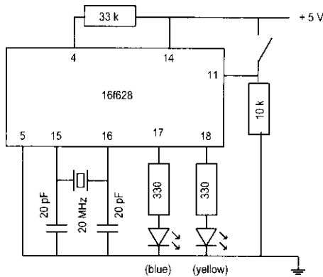
Figure 196. Demo project for the 16F628.
