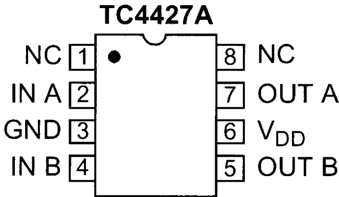
Figure 176. Connections of the TC4427A.
