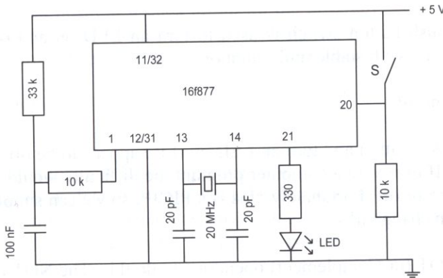
Figure 27. Timer.
