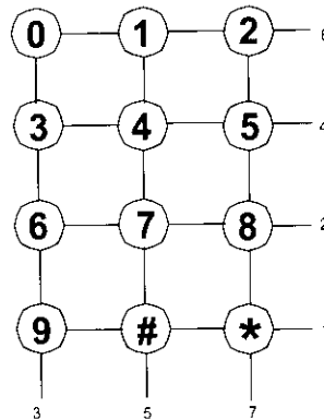
Figure 31. Key arrangement on the keypad.
