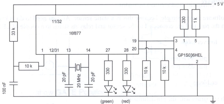
Figure 94. Tilt sensor schematic.
