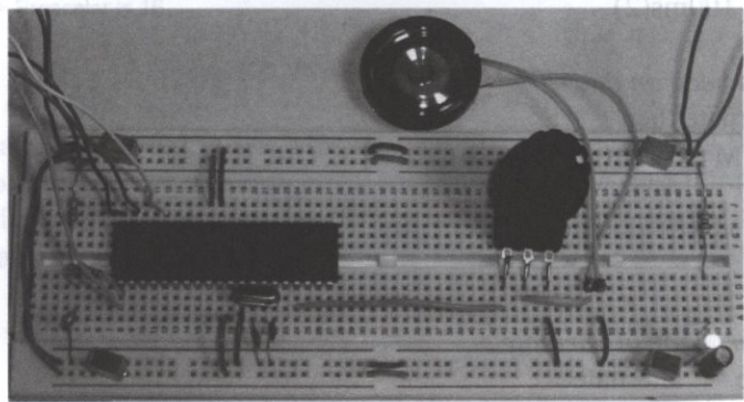
Figure 100. Beep.
