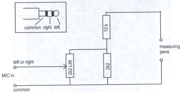
Figure 10. Interface for mic or line input of a soundcard on a PC.
