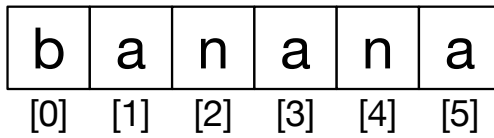
Figure 6.1: String Indexes
